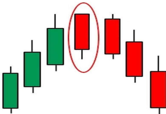
Bearish Belt Hold
